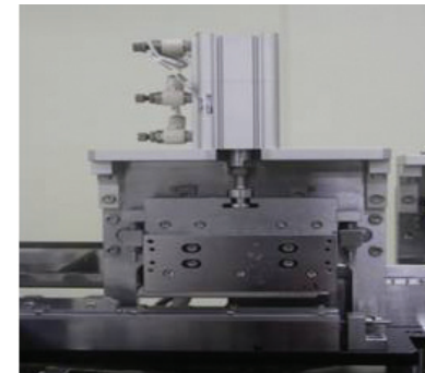
Cutting Unit
